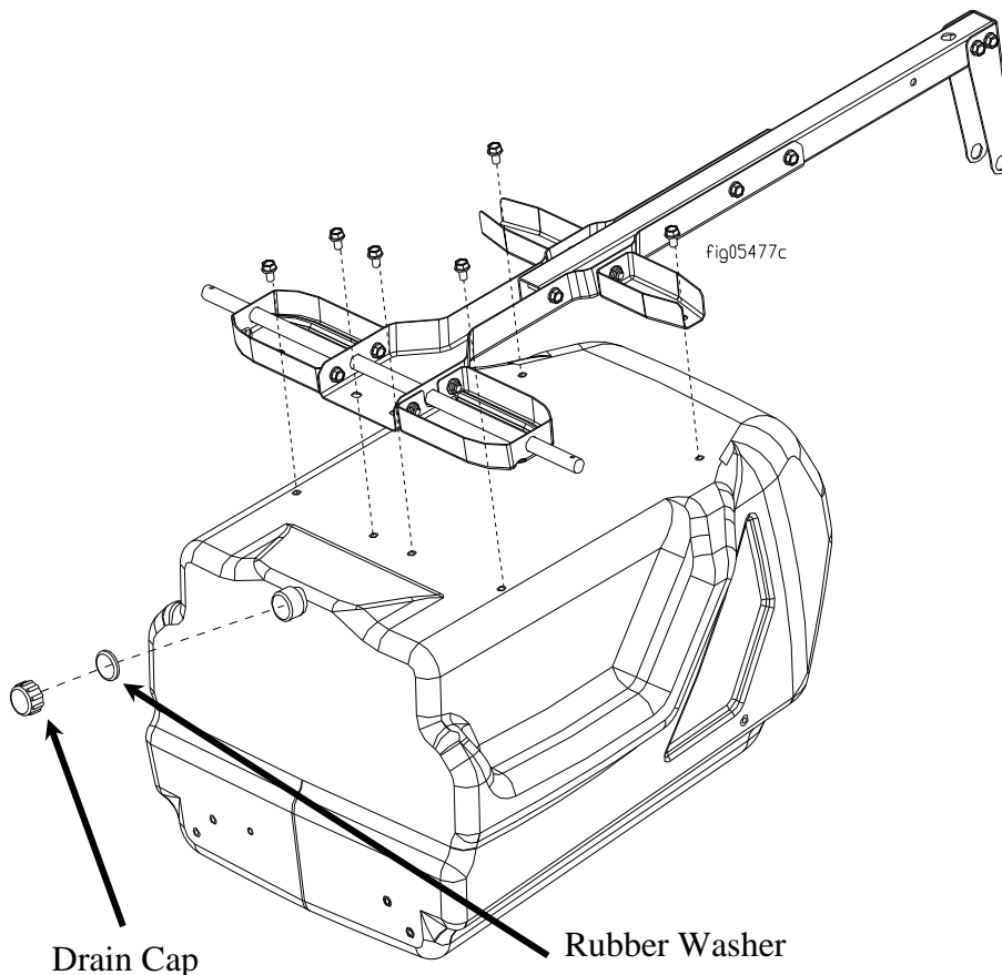
5/16" x 1/2" Bolt Qty 6 82014
